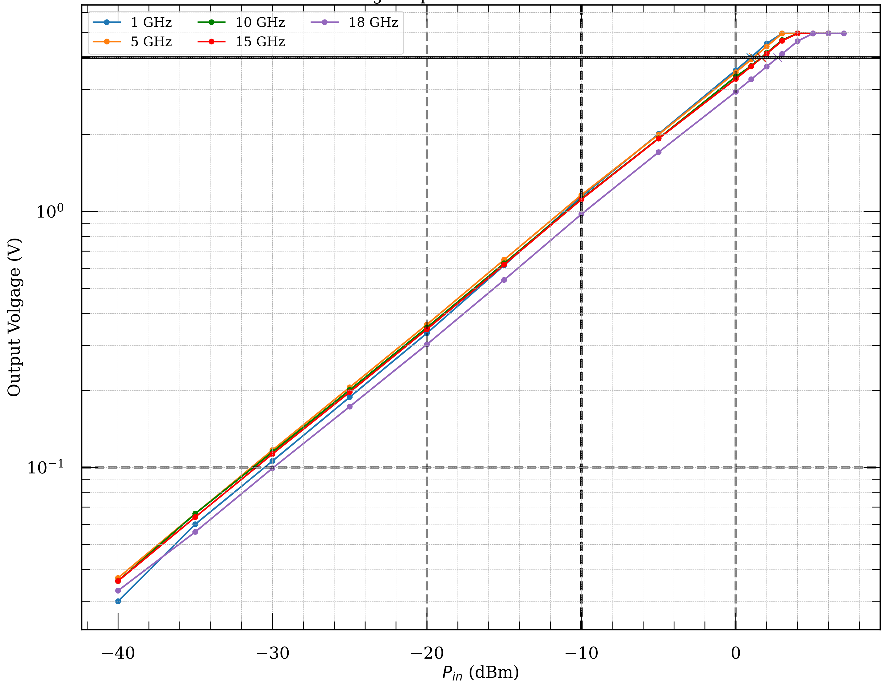
Measured voltage-to-power curve of detector module008
